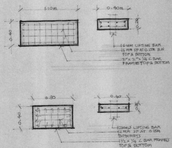
DETAIL M.H. COVER
