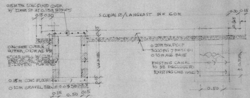
ROAD CROSS-SECTION FIXED COVER LANGKA ST. / S. CUEVAS ST.
