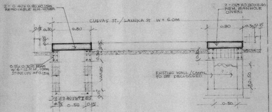
ROAD CROSS-SECTION AT MANHOLE LANGKA ST. / S. CUEVAS ST.
